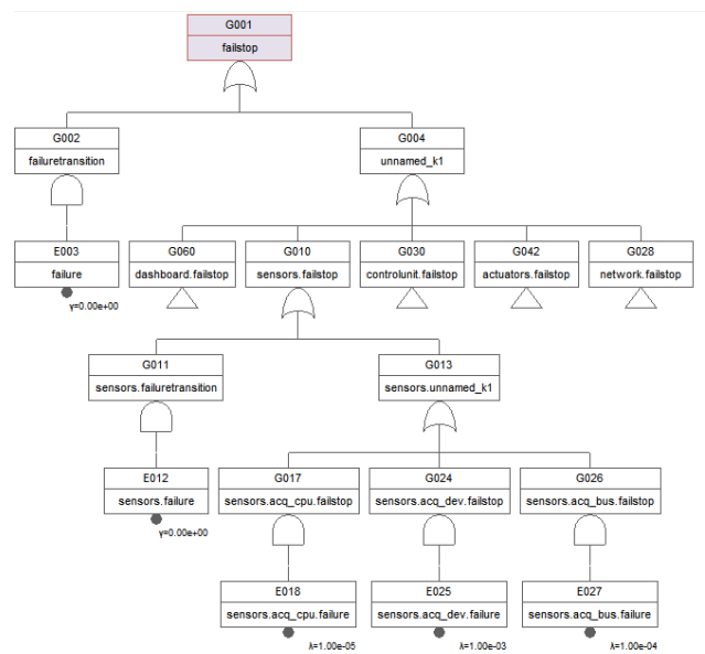
Figure 6: Fault tree in Arbore Analyste
