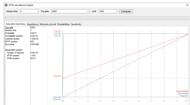
Figure 7: MTBF computation in Arbore Analyste
